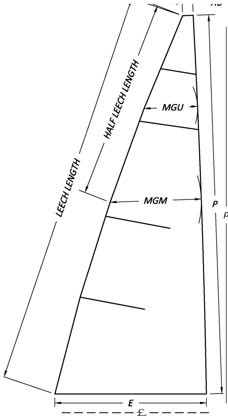
MAINSAIL MEASUREMENTS
